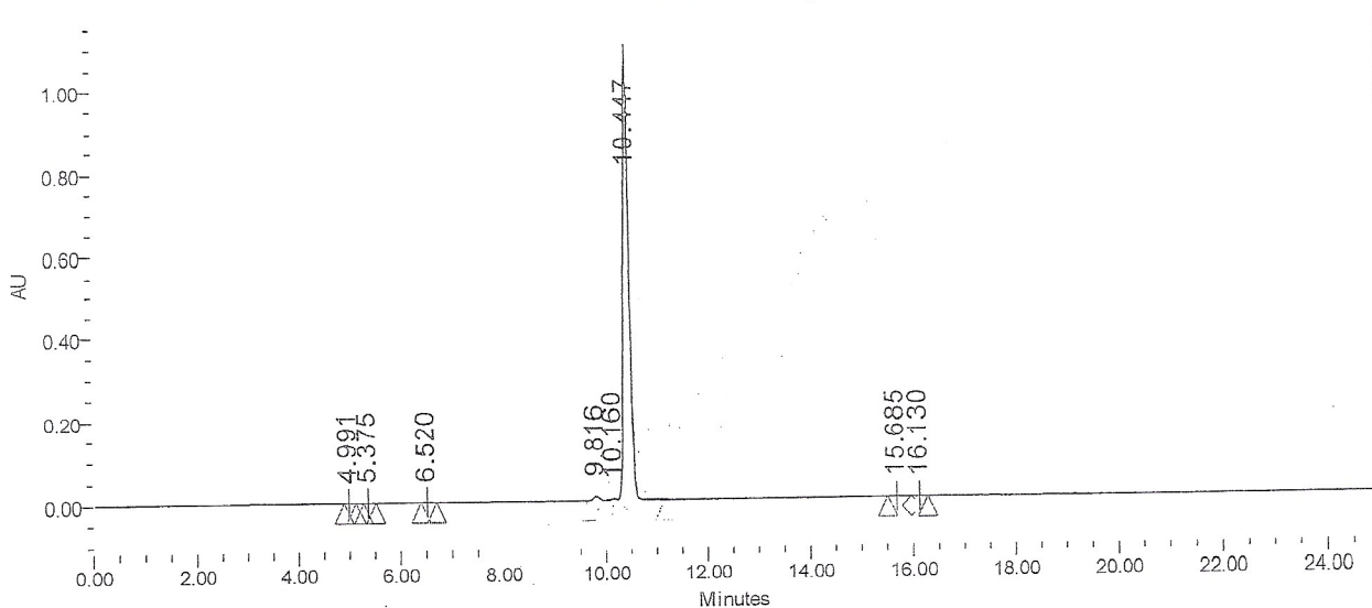
Auto-Scaled Chromatogram
